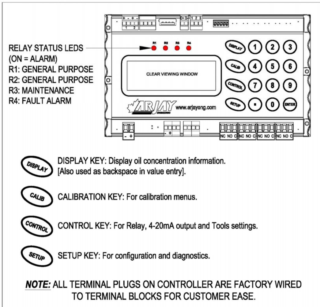
Figure 4 - USER INTERFACE
