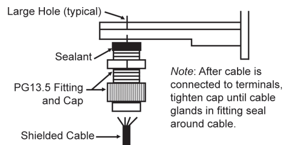
Figure 3-14. Inserting Shielded Interconnect Cable Through PG13.5 Fitting and Cap.
